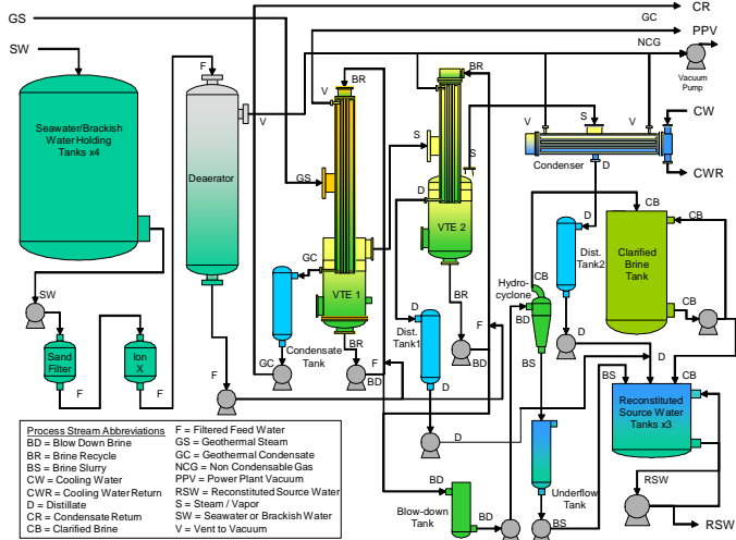
VTE Pilot Plant Schematic, Figure 3.
